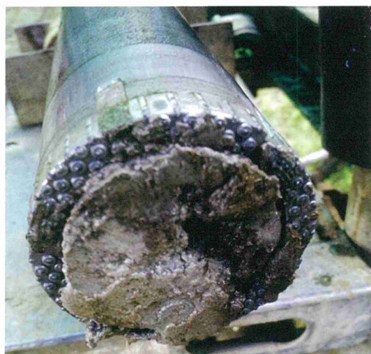
“粘土”掘削
